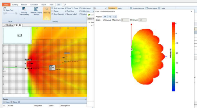
2D and 3D RSRP Broadcast Antenna Beam Prediction
