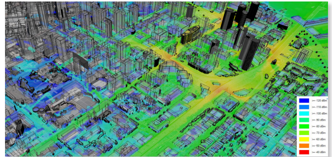
3D visualisation of indoor and outdoor network coverage
